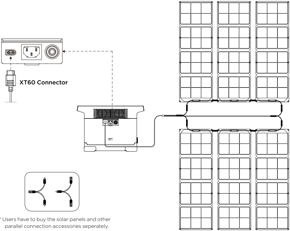
SOLAR PANEL-21.6V X6
