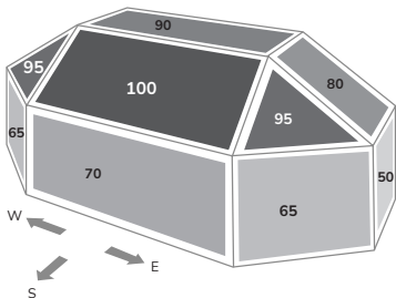
Northern hemisphere
