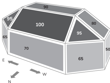
Southern hemisphere
